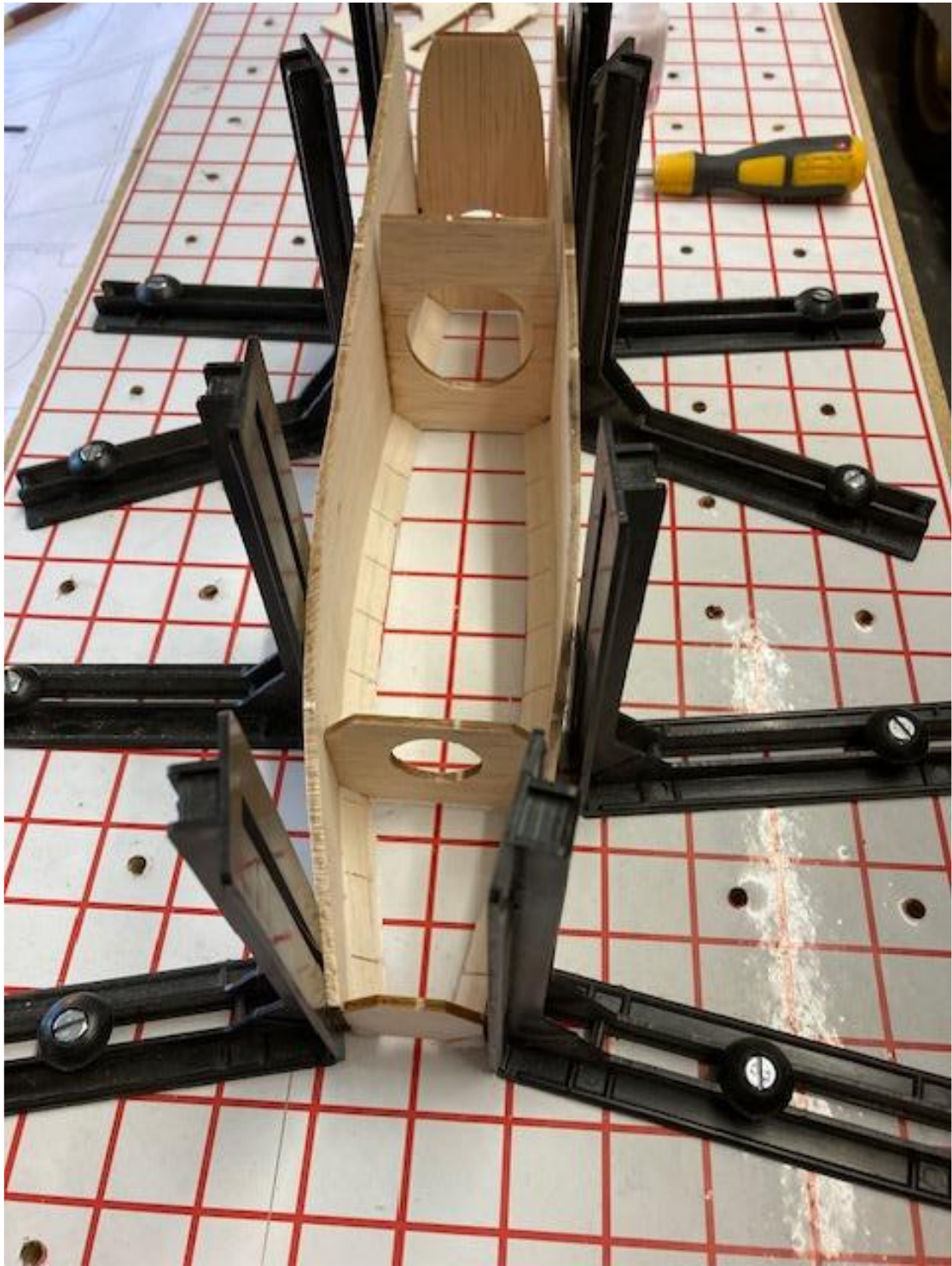
Front Fuselage
