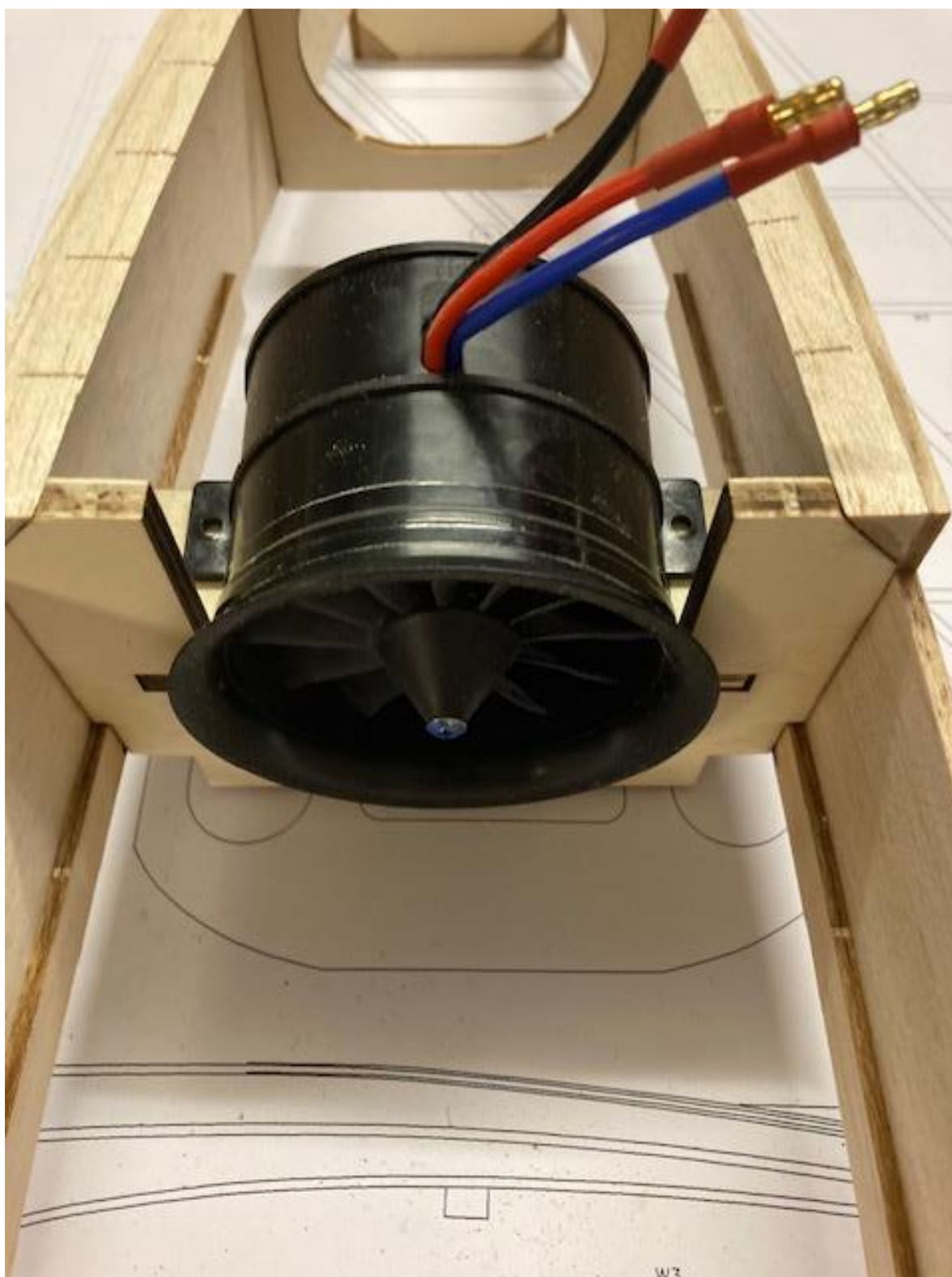
70mm PowerFun 4S EDF unit
