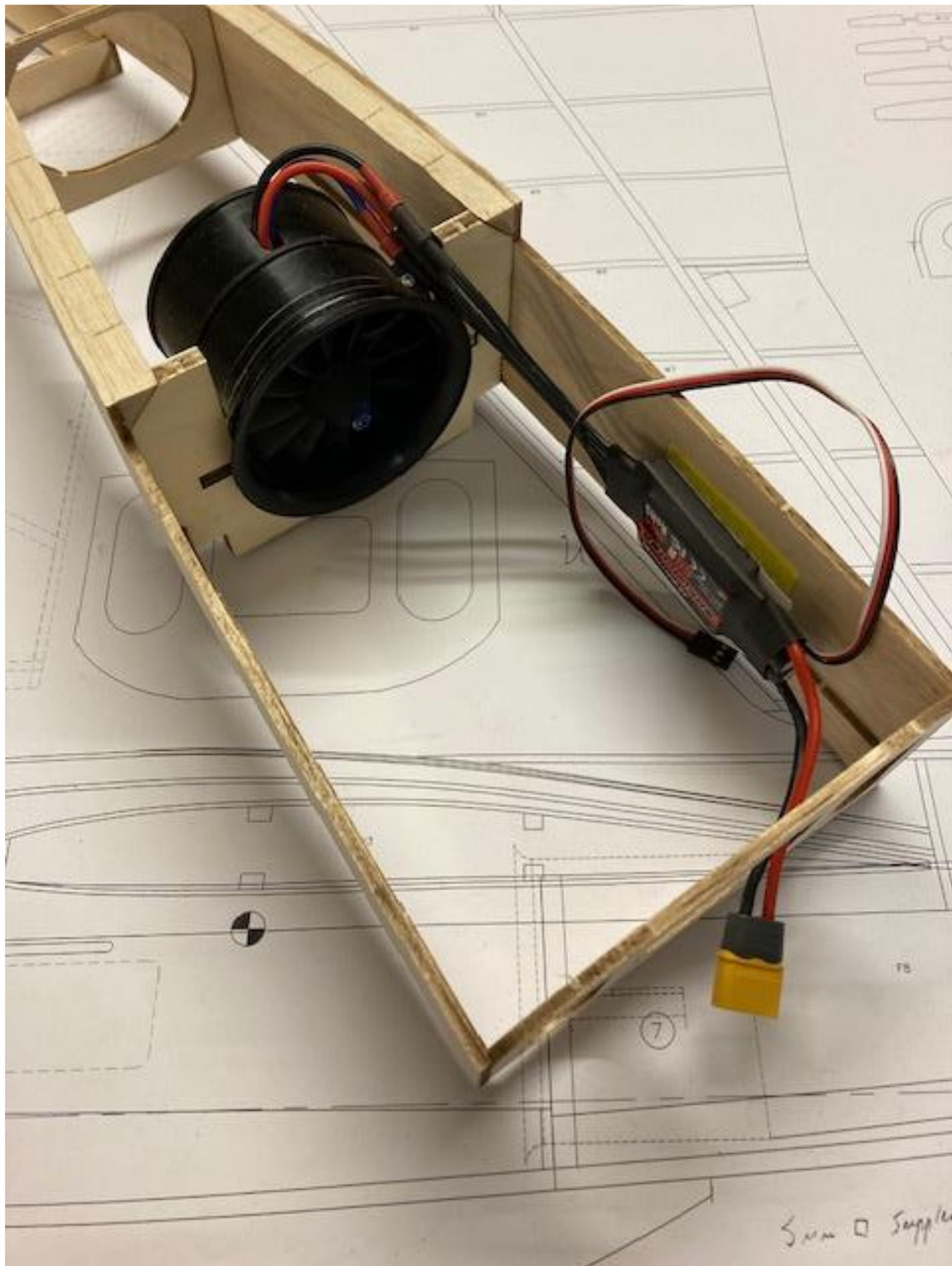
Test/use with 60amp ESC
