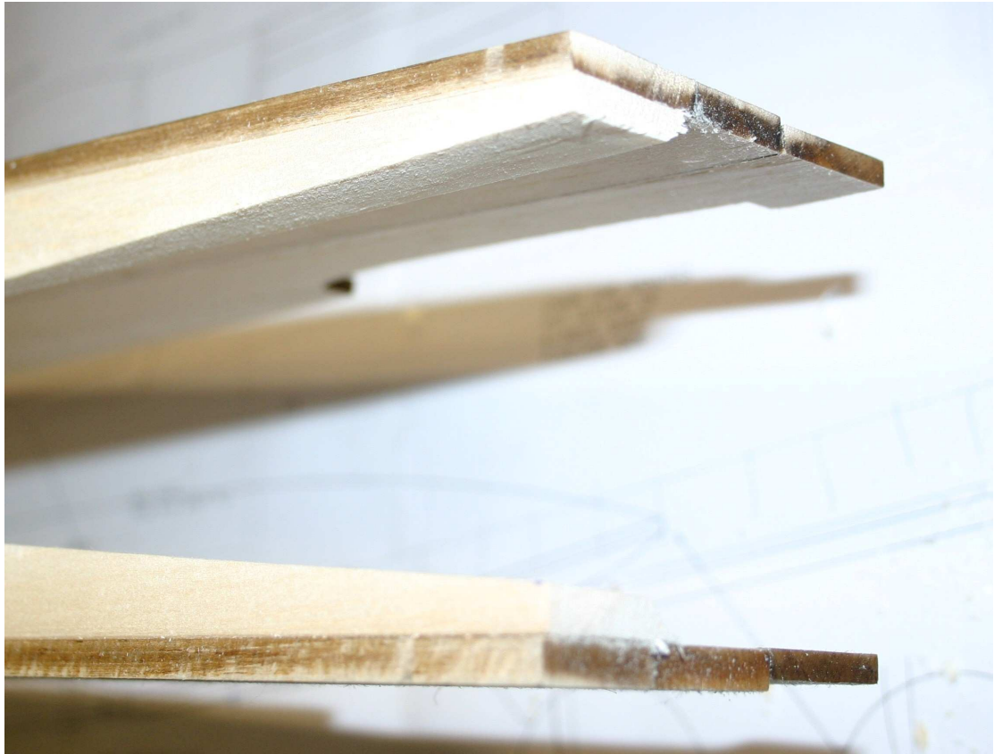
Feather triangle at rear of fuselage so tailpost fits snugly
